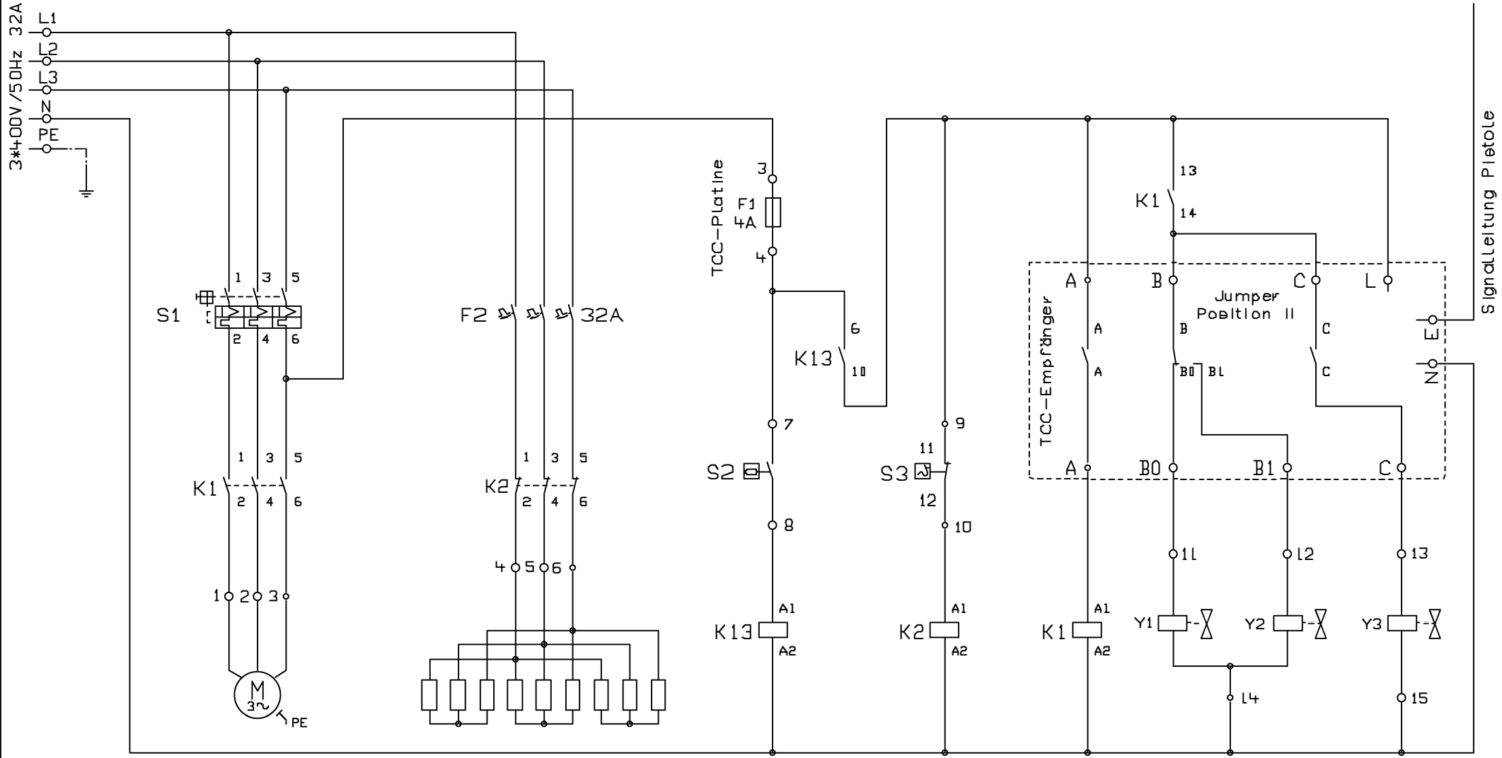
HD-Pumpe
