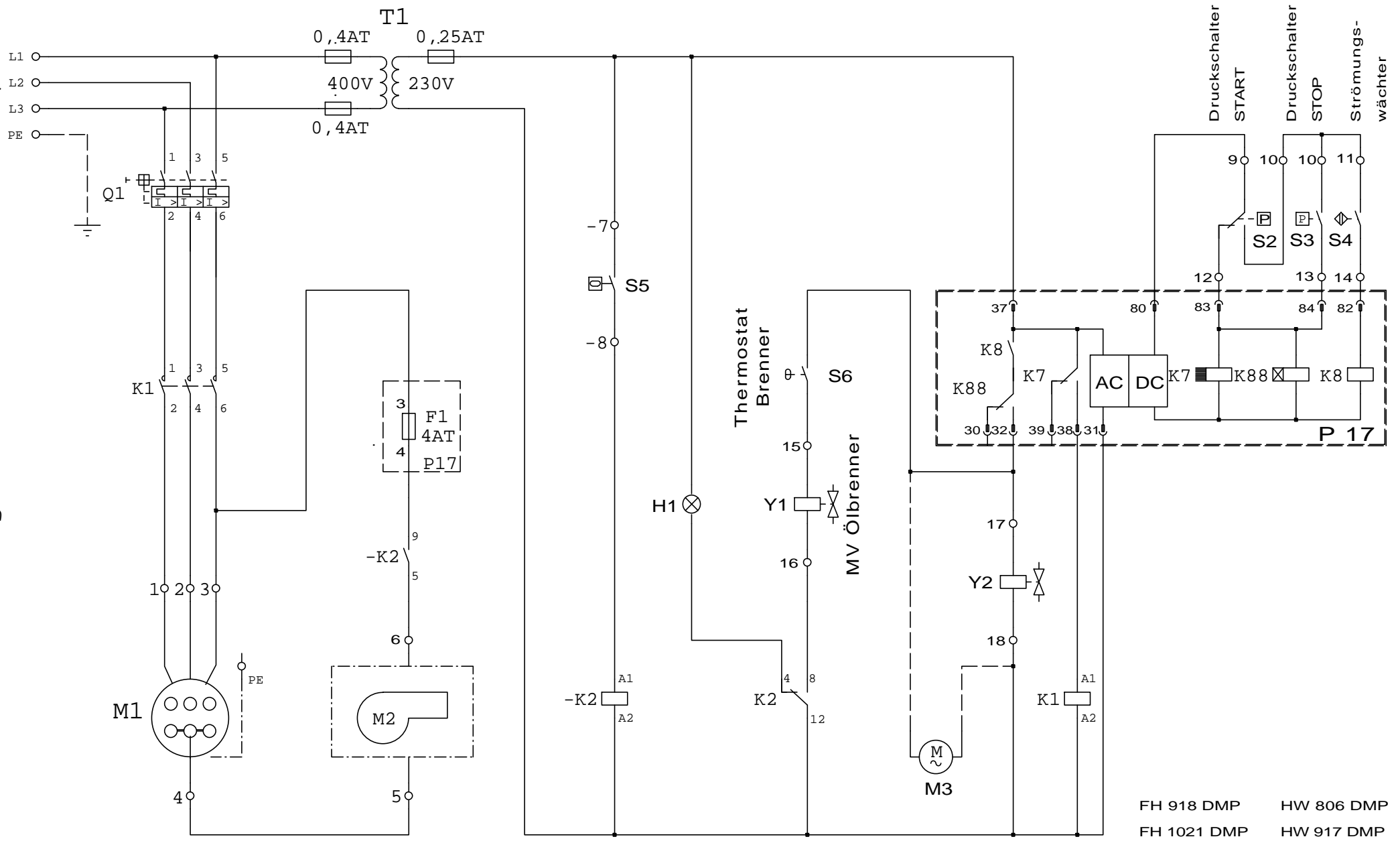
Motor-Pumpe
