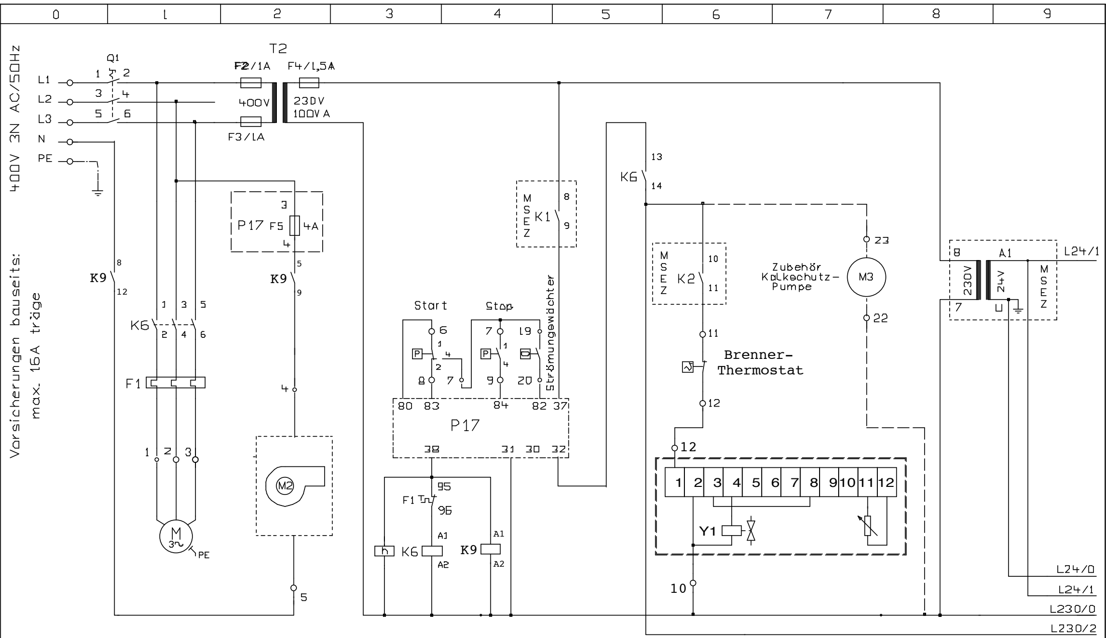
Motor-Pumpe
